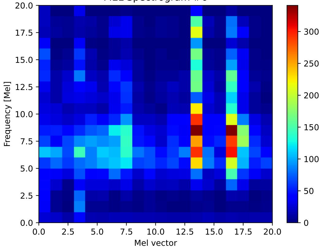
MEL Spectrogram #6
